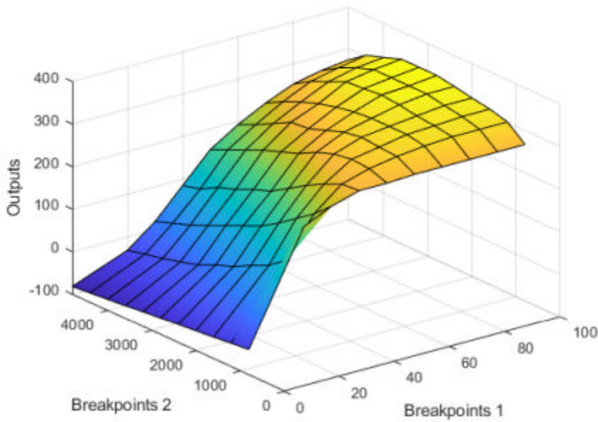
Figure 1.1. engine torque (:,:)
